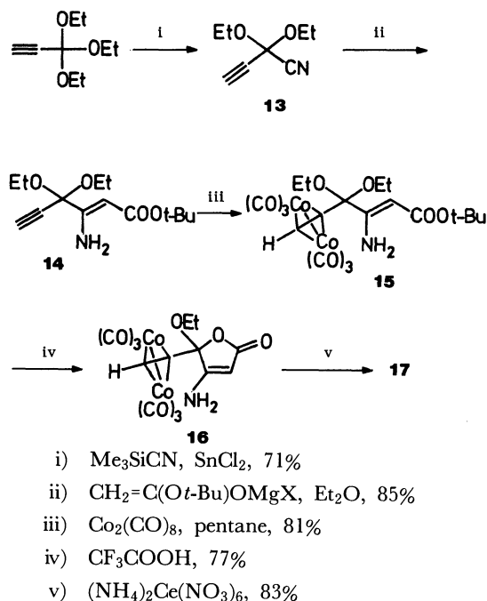
Scheme 4.
